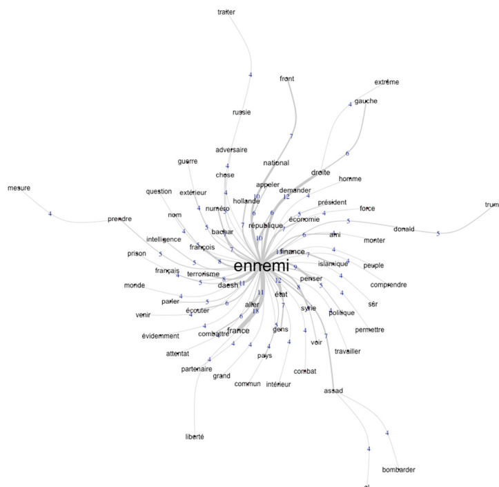
Figure 4. Similarity analysis.
