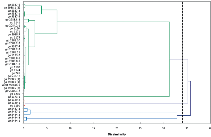
Fig. 5 — Grouping of different parts and fragments of the West Mebon Viṣṇu, and the two hands ga 5444 and ga 5447, according to their metal composition. Clustering made on the 4 first components of a principal components analysis (PCA) carried out on 11 chemical elements (Ag, As, Au, Bi, Co, Fe, Ni, Pb, Sb, Se, Sn). Dendrogram: D. Bourgarit.
