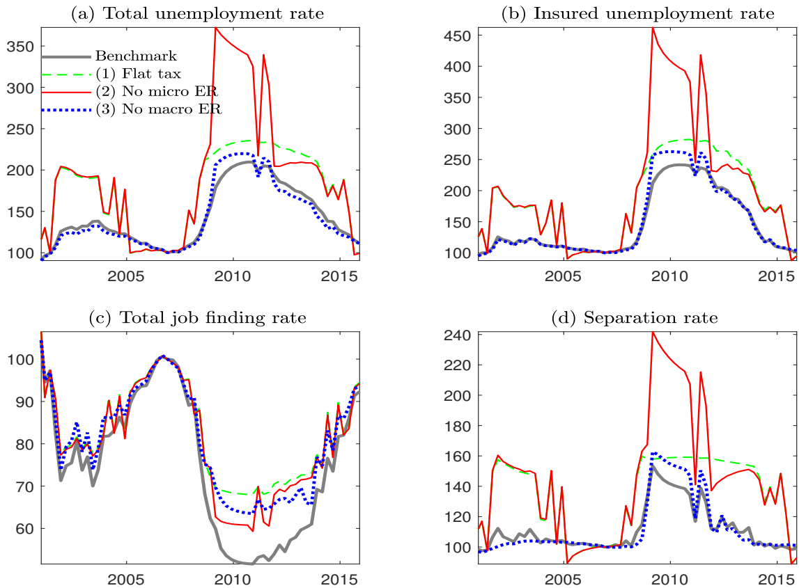
Figure 8: Counterfactual simulations
