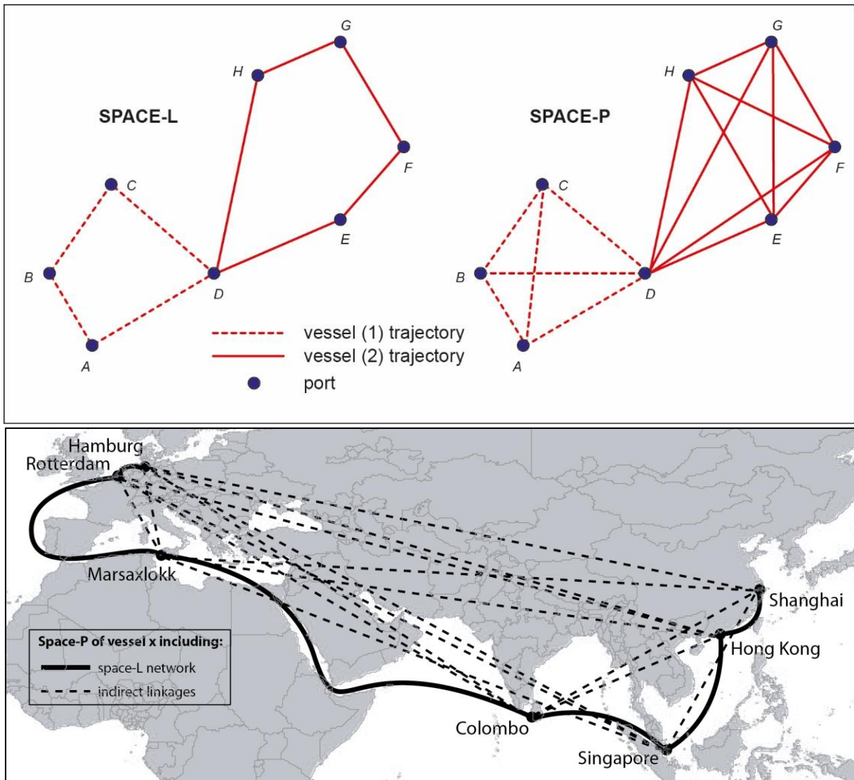
Figure 2: Topologies of the liner shipping network
