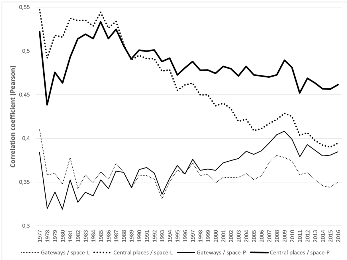
Figure 5: Port-city correlation under different network topologies, 1977-2016
