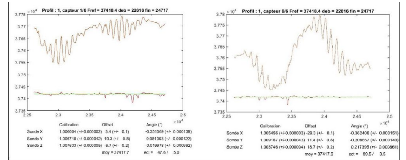
Figure 3: First test - Compensation/calibration of the magnetometer with the highest standard deviation after correction that correspond to the magnetometer placed at the extremities of the stick (R. Al Khatib Alkontar, H. Reiller – MAFTOr/IPGS-EOST).
