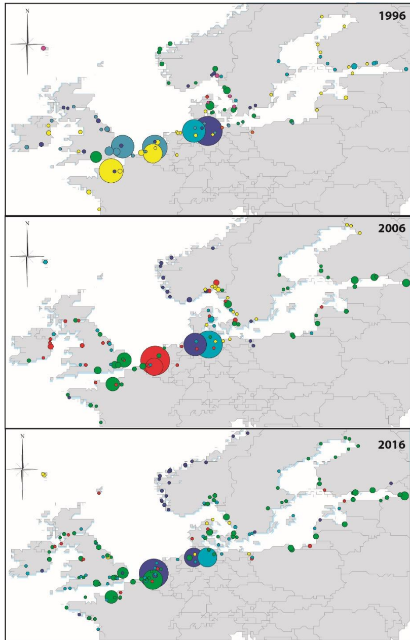
Figure 4: Cluster identification among North European container ports, 1996-2016
