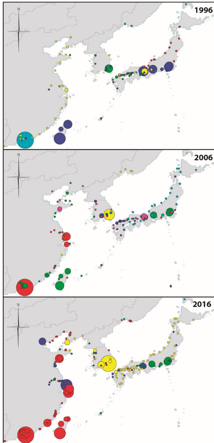
Figure 5: Cluster identification among Northeast Asian container ports, 1996-2016
