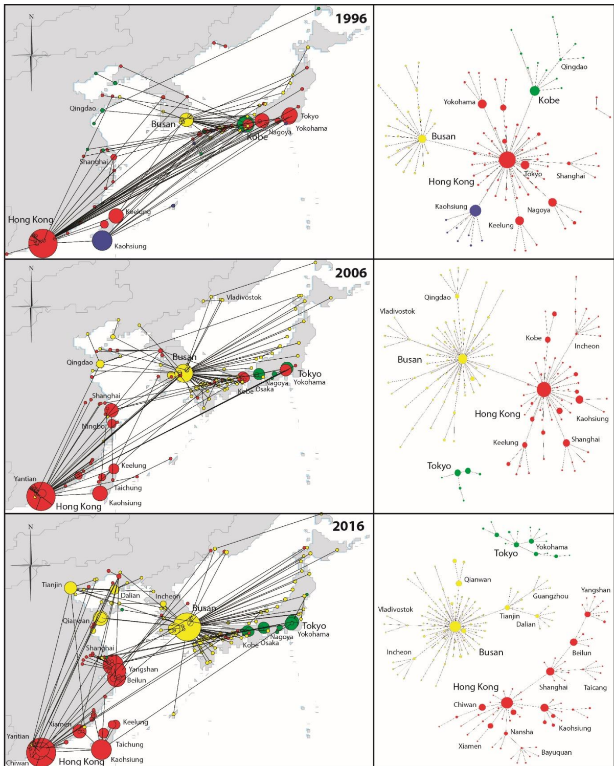
Figure 3: Single linkage analysis of Northeast Asian container flows, 1996-2016
