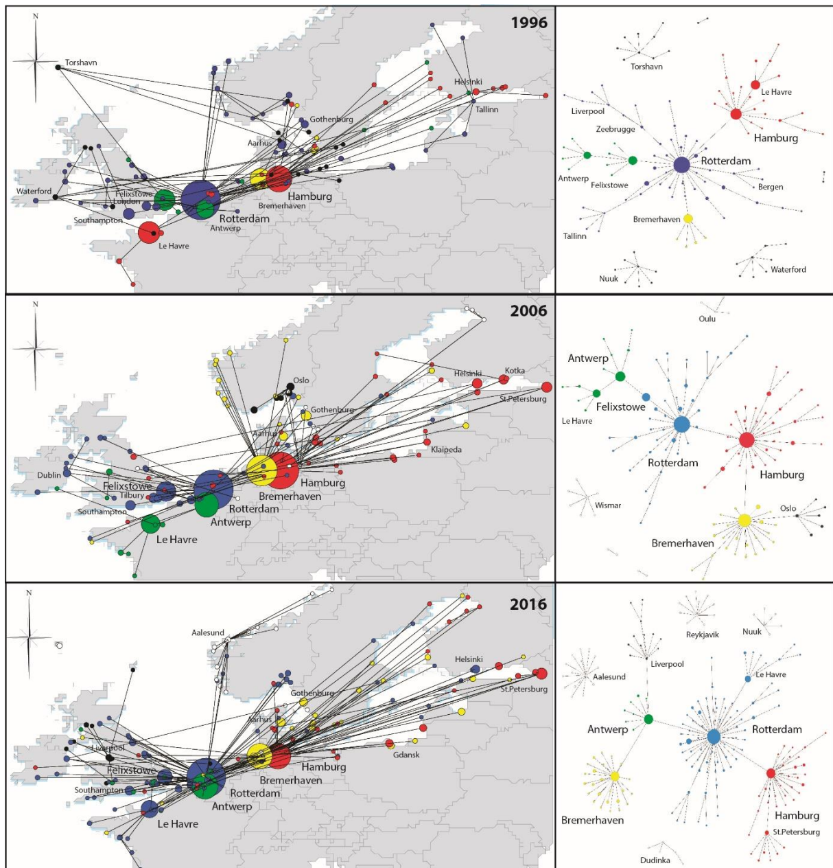
Figure 2: Single linkage analysis of North European container flows, 1996-2016
