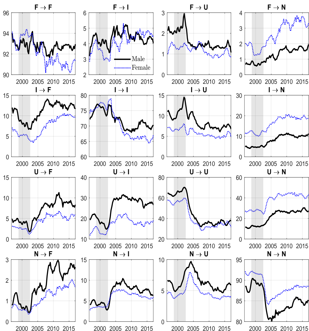
Figure 13: Transition probabilities - Males vs Females
