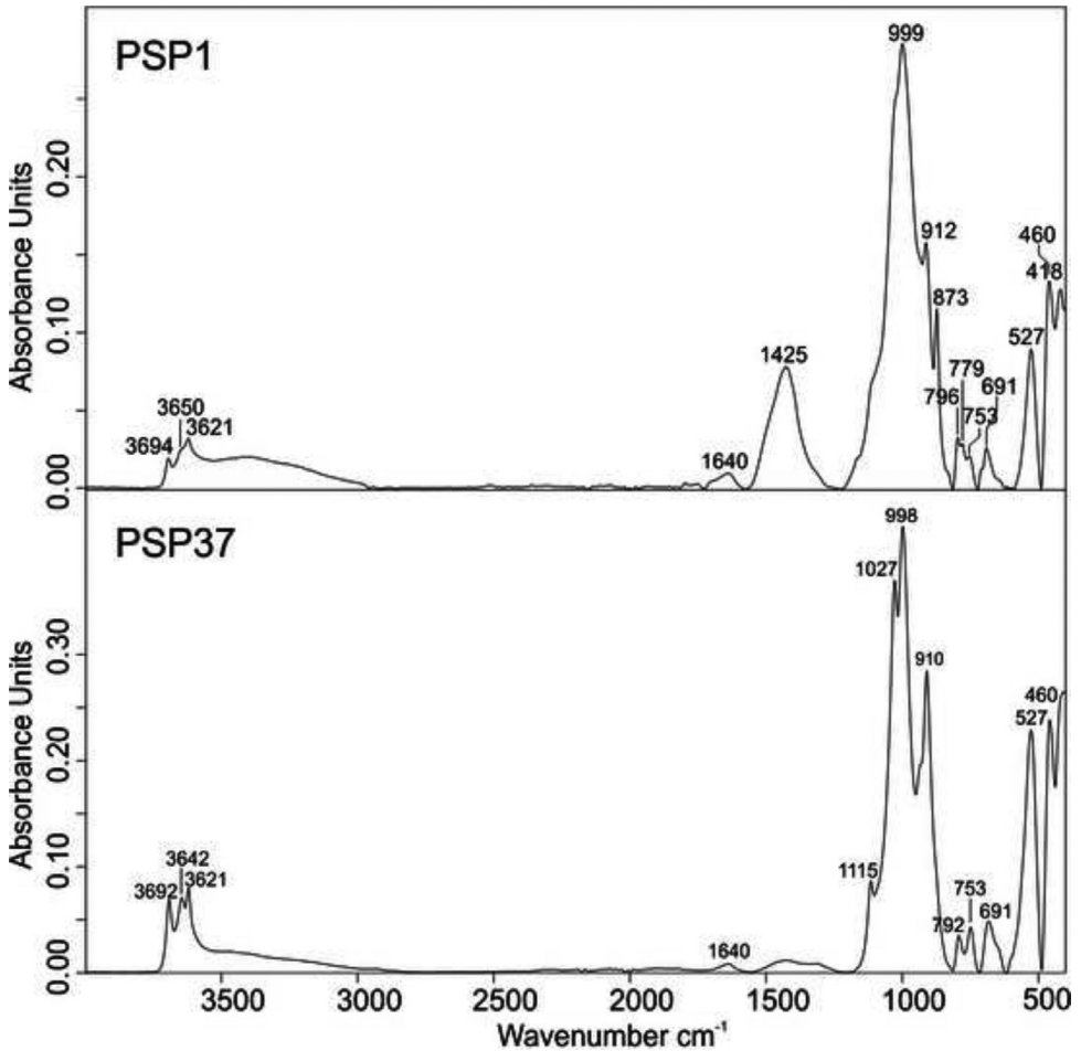
Fig. 7. ATR-FTIR spectra of the ceramic slip scratched from the sample PSP1 (a) and of the reddish deposit recovered in the workshop (PSP37).
