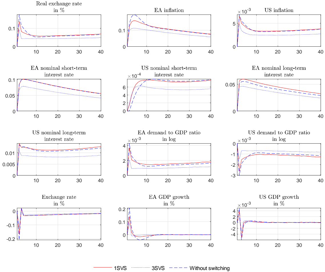
Figure 9: Unconditional IRFs to a positive EA monetary policy shock (one standard deviation).
