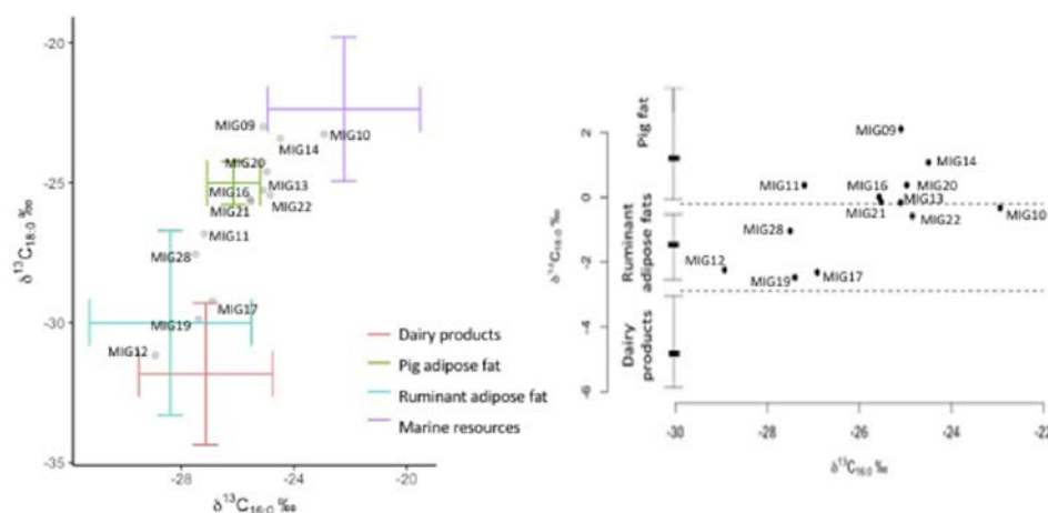
Figure 5. \delta^{13}\text{C} values of \text{C}_{16:0} and \text{C}_{18:0} n-alkanoic acids (a) and \delta^{13}\text{C} values of \text{C}_{16:0} and \Delta^{13}\text{C} ( \delta^{13}\text{C} \text{ C}_{18:0} - \delta^{13}\text{C} \text{ C}_{16:0} ) n-alkanoic acids (b) obtained from Mines de Gavà site. The 68% confidence ellipses are based on modern reference fats extracted from the literature (See Supplementary Table 2).
