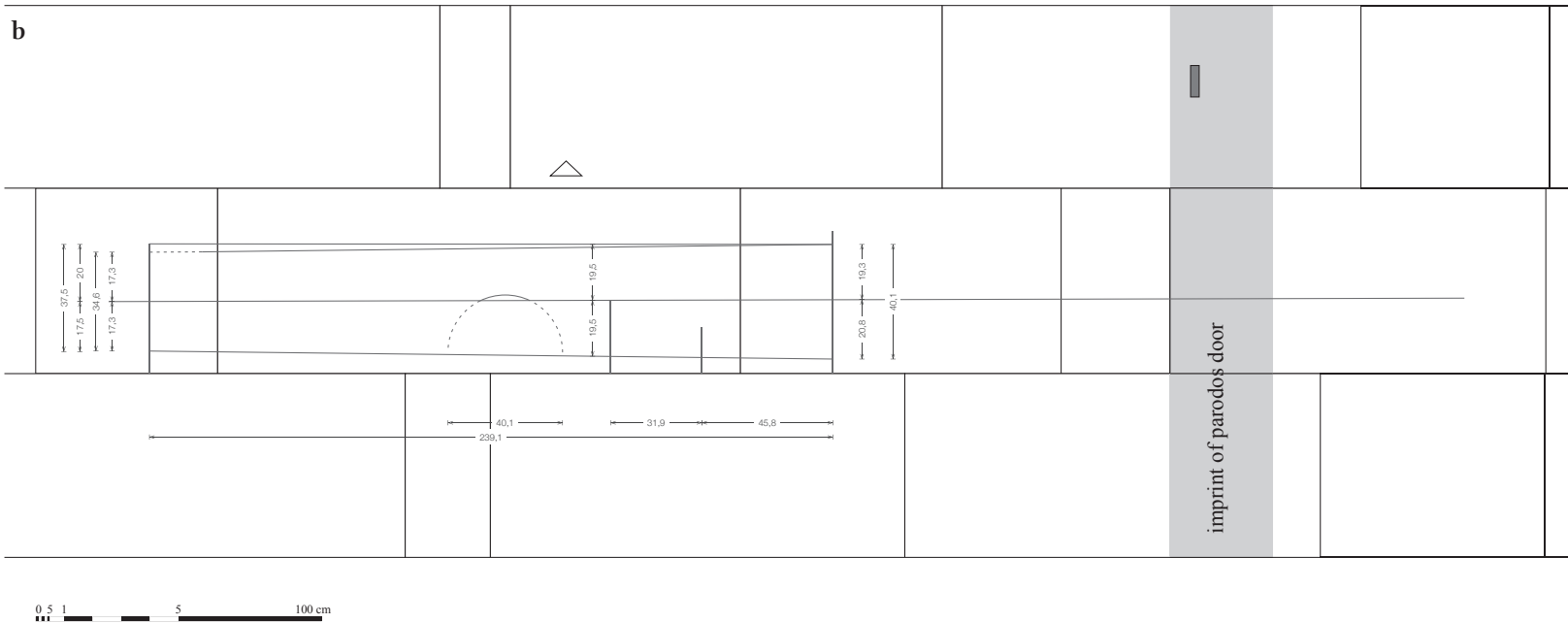
FIGURE 3.12A–C Larisa, theatre: (a) proskenion façade in the foreground and western retaining wall in the background; (b) blueprint of the proskenion semi-columns; (c) setting lines on the stylobate of the scene building (white lines overlaid) PHOTOGRAPHS AND DRAWING ARE BY THE AUTHOR
