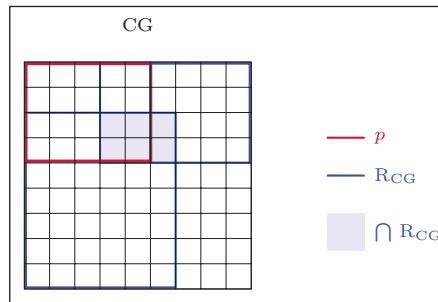
Figure 9: Non-homogeneity of \cap R_{cg} with respect to p .
