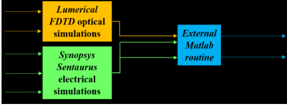
Figure 1 Block diagram of Photon Detection Probability estimation
