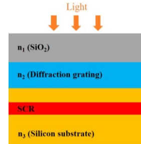
Figure 5 Simplified equivalent optical schematic of SPAD structure
