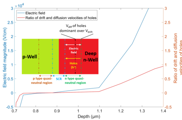
Figure 3 Profiles of electric field and ratio of drift and diffusion velocities of holes at the n-side limit of SCR
