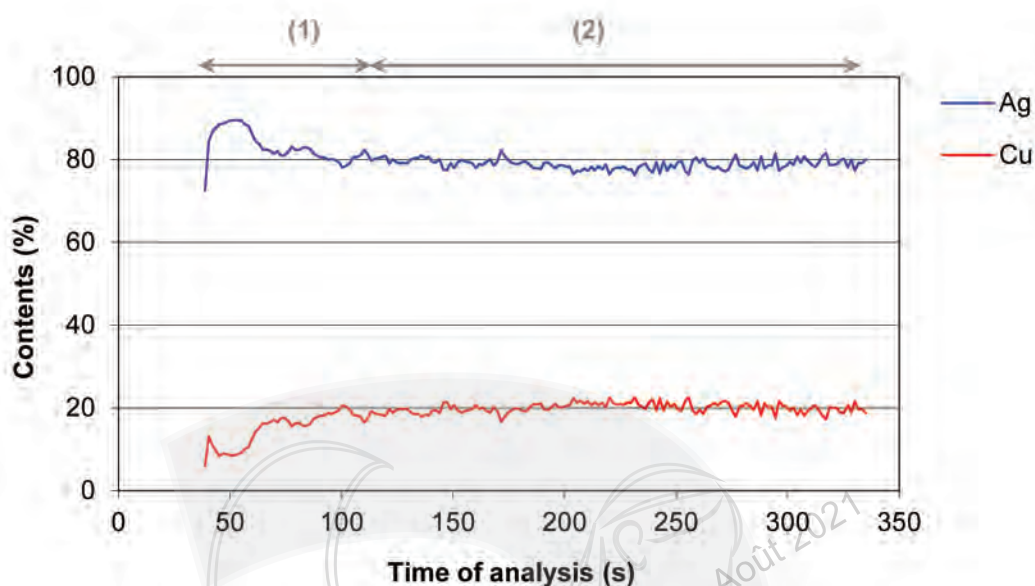
Fig. 1. LA-ICP-MS depth profile mode carried out on a Thessalian koinon coin (BnF FG 11). (1) Perturbed surface. (2) "Inner part" of the coin.
