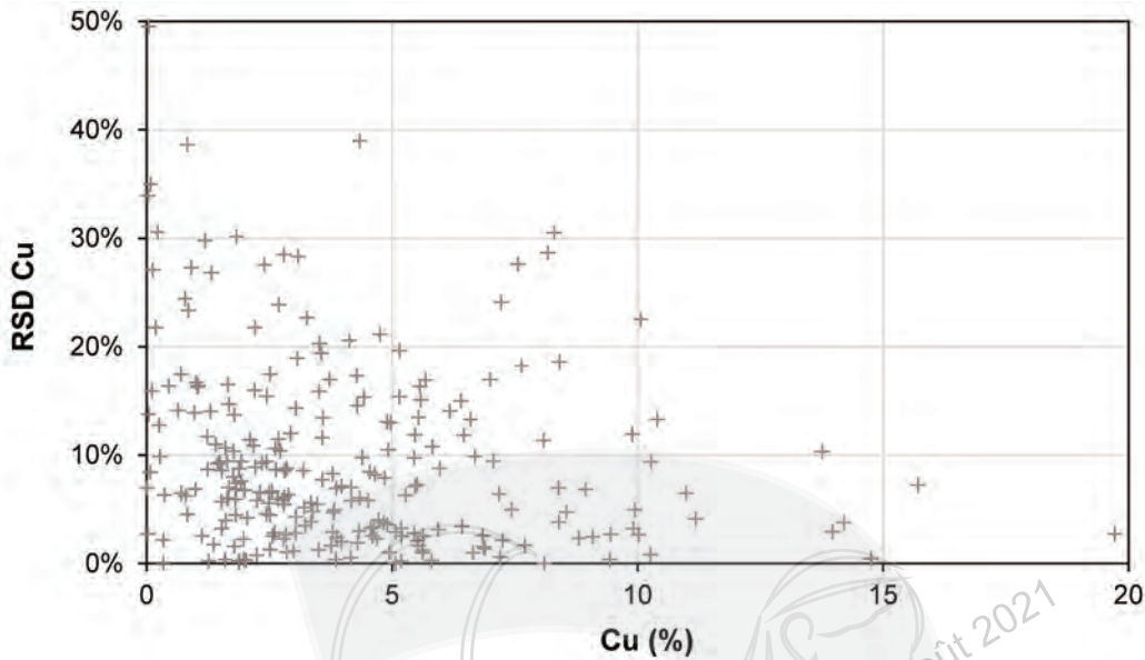
Fig. 3. Relative standard deviations (RSD) of copper contents against the average copper contents for all the 251 Greek Hellenistic silver coins analysed by LA-ICP-MS in the framework of the KOINON project.
