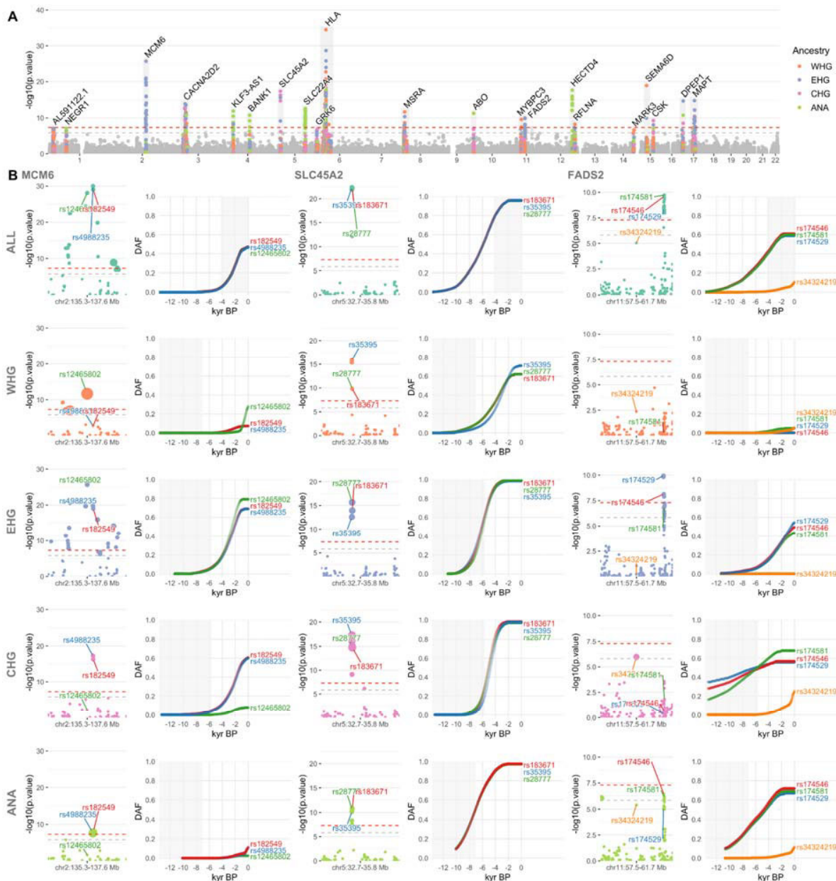
922 Fig 7. Genome-wide selection scan for trait associated variants. A) Manhattan plot of p-values from selection scan 923 with CLUES, based on a time-series of imputed aDNA genotype probabilities. Twenty-one genome-wide significant 924 selection peaks highlighted in grey and labelled with the most significant gene within each locus. Within each sweep, 925 SNPs are positioned on the y-axis and coloured by their most significant marginal ancestry. Outside of the sweeps, 926 SNPs show p-values from the pan-ancestry analysis and are coloured grey. Red dotted lines indicate genome-wide 927 significance ( p < 5e-8 ), while the grey dotted line shows the Bonferroni significance threshold, corrected for the number 928 of tests ( p < 1.35e-6 ). B) Detailed plots for three genome-wide significant sweep loci: (i) MCM6, lactase persistence; 929 (ii) SLC45A2, skin pigmentation; and (iii) FADS2, lipid metabolism. Rows show results for the pan-ancestry analysis 930 (ALL) plus the four marginal ancestries: Western hunter-gatherers (WHG), Eastern hunter-gatherers (EHG), Caucasus 931 hunter-gatherers (CHG) and Anatolian farmers (ANA). The first column of each loci shows zoomed Manhattan plots of 932 the p-values for each ancestry (significant SNPs sized by their selection coefficients), and column two shows allele
