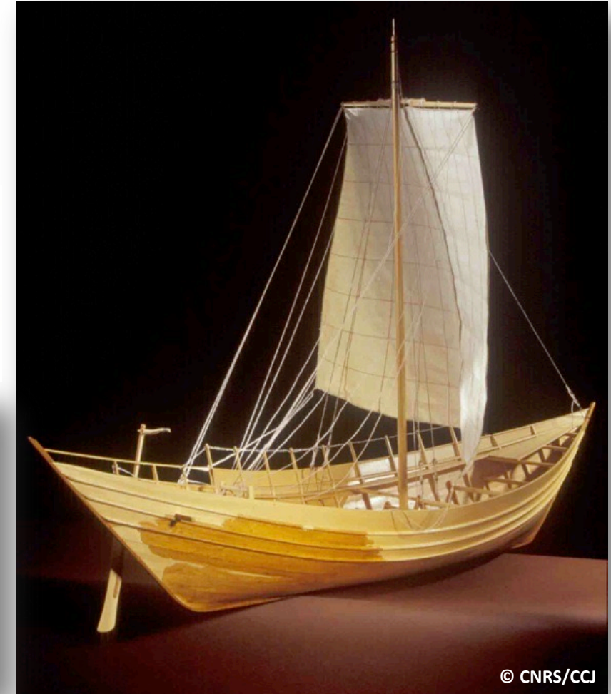
Jules Verne 7, tenon-and-mortise joints with residual stitching and sewn repairs
