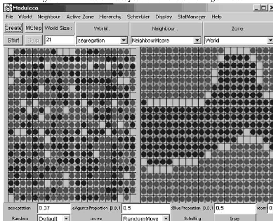
Figure 12: Moduleco adaptation of the Schelling's model.
