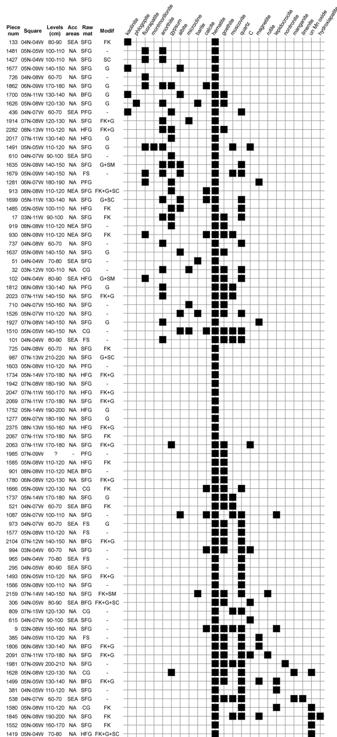
Figure 6. Seriation analysis of minerals identified by micro-Raman spectroscopy on ochre pieces from Porc-Epic Cave. Num number, acc accumulation, mat material, modif modifications, SEA southeastern area, NEA northeastern area, NA not applicable, SFG soft fine-grained, BFG banded fine-grained, HFG hard fine-grained, CG coarse-grained, FS ferruginous sandstone, PFG platy fine-grained, FK flaking, SC scraping, G grinding, SM smoothing, C carbon, un undetermined.
