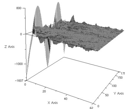
Fig. 10. Spatial scattering function of the indented surface.
