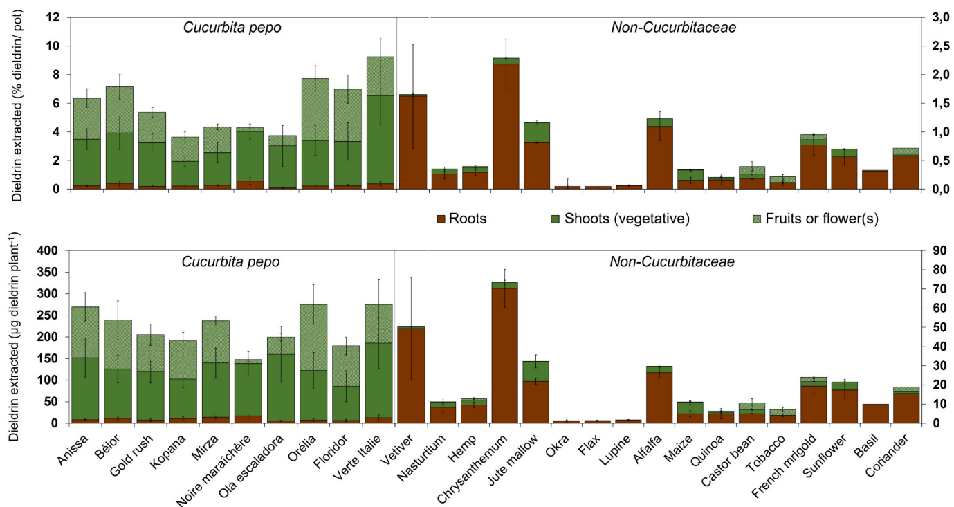
Fig. 5. Dieldrin extracted in % of dieldrin present in the potted soil (top) and dieldrin amount extracted (bottom) by the fruits or flowers (green striped bar graph), vegetative shoots (uniform green bar graph), and roots (brown bar graph) for the C. pepo varieties and the non-Cucurbitaceae species. Left scale for all the C. pepo varieties and vetiver, right scale for all the other non-Cucurbitaceae species. Mean value \pm SE ( n = 4 , except for C. pepo fruits for which n is indicated in Fig. 3).
