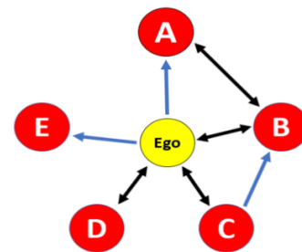
Figure 1: A directed graph network with unidirectional (blue) and bi-directional (black) edges
