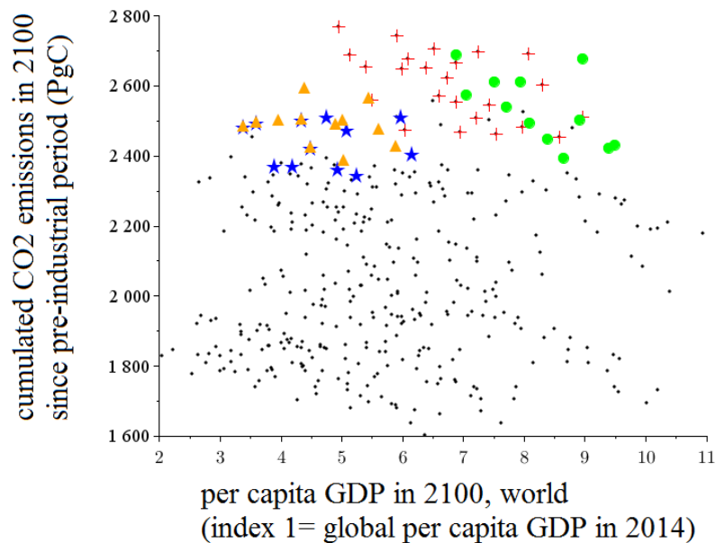
Figure 17 : The 432 scenarios plotted according to the global per capita GDP in 2100 (X-axis) and the global cumulated CO 2 emissions since the pre-industrial period (Y-axis). Families of scenarios uncovered by PRIM analysis are materialized with red crosses (family 1), blue stars (family 2), green circles (family 3) and orange triangles (family 4). (Guivarch et al., 2016).
